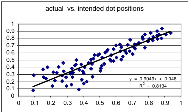
Figure 2b: Plot of dot positions
